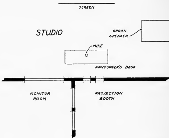
FIG. 2. General plan of studio and equipment rooms.
